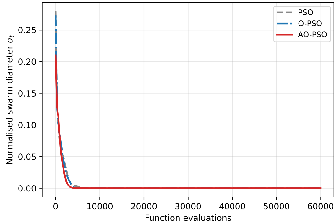
Swarm diversity on Rastrigin (D=30)
