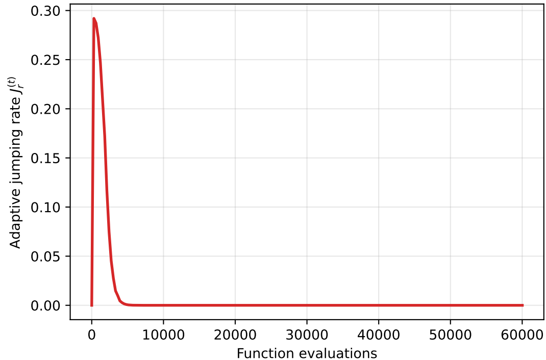
AO-PSO: J_r falls as the swarm converges
