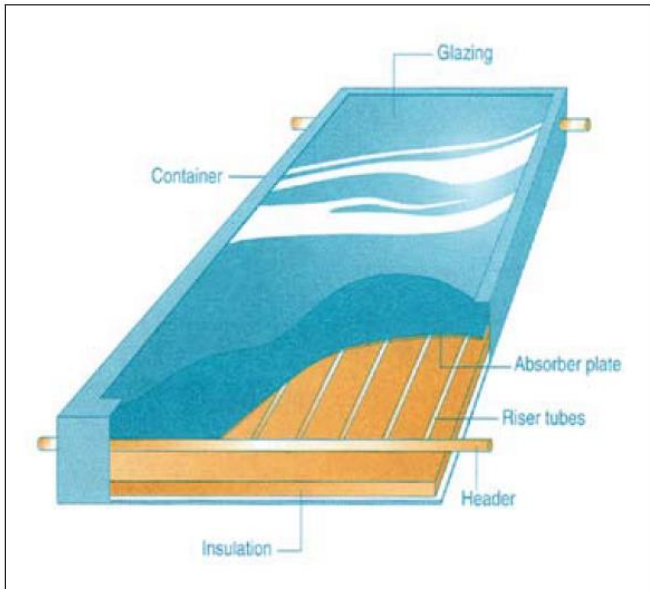
Figure 9: System Schematic for Glazed Flat-Plate Solar Collector.
