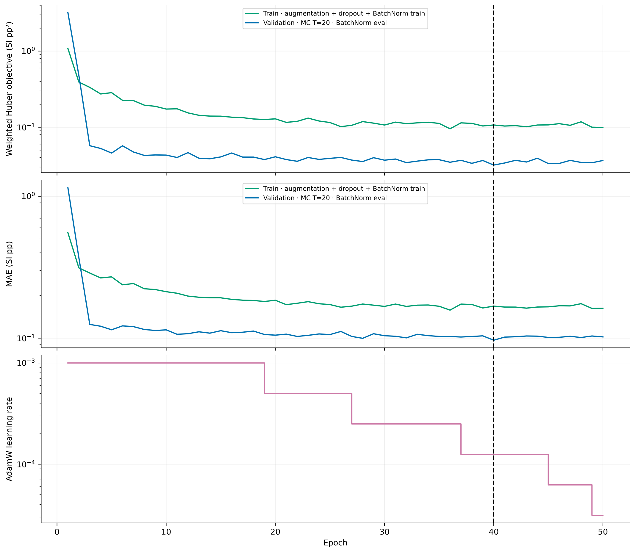
Coronium V3.1 · Training and validation · selected epoch 40 of 50 Phase 1.5 weights promoted as V3.1 · log axes; raw SI targets · train/validation protocols differ
