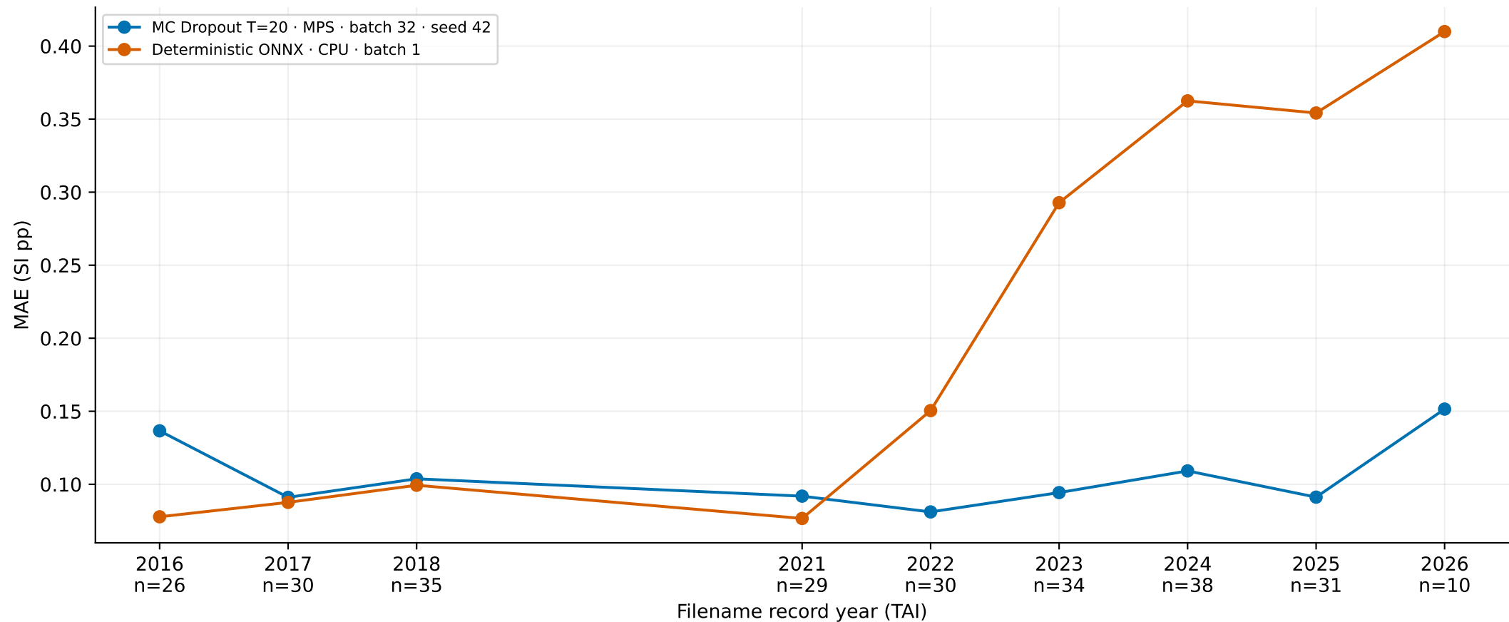
Coronium V3.1 · Descriptive error by record year · random selection validation Selection validation; no untouched test or temporal generalization
