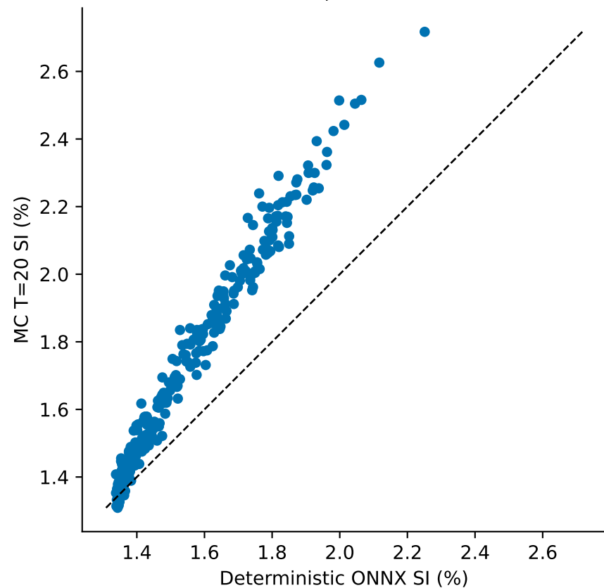
Paired predictions
