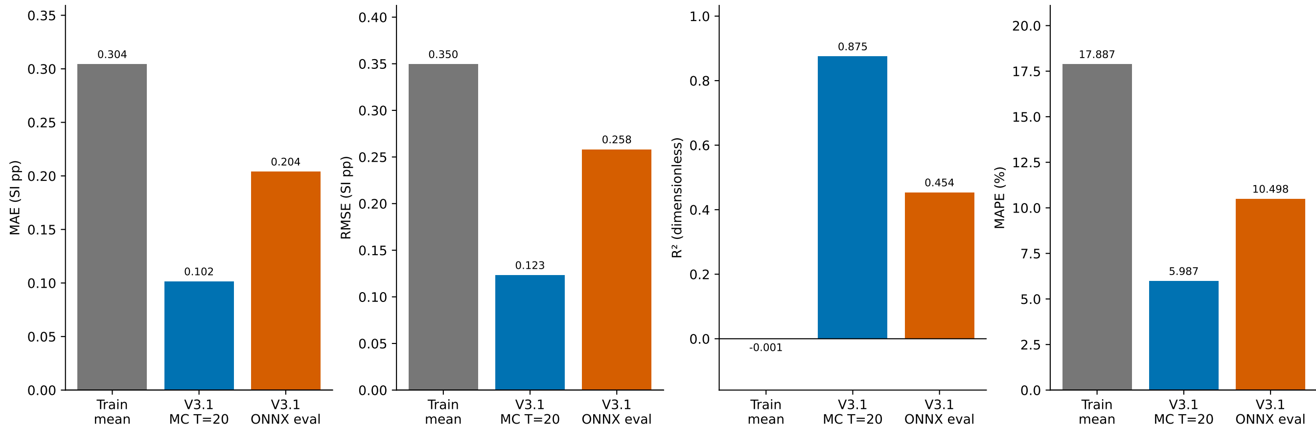
Coronium V3.1 · Constant training-mean baseline on the same 263 observations Selection validation; no untouched test or temporal generalization
