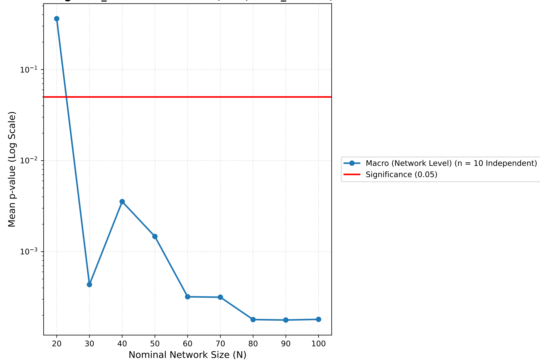
Congenial_Count: Left Users (K=4, Hide_Shared)
