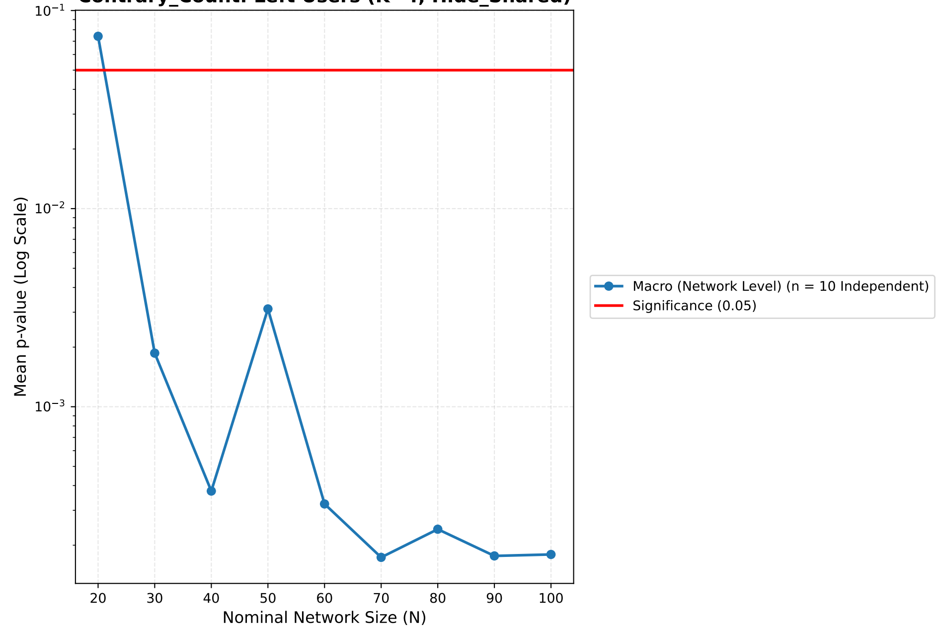
Contrary_Count: Left Users (K=4, Hide_Shared)
