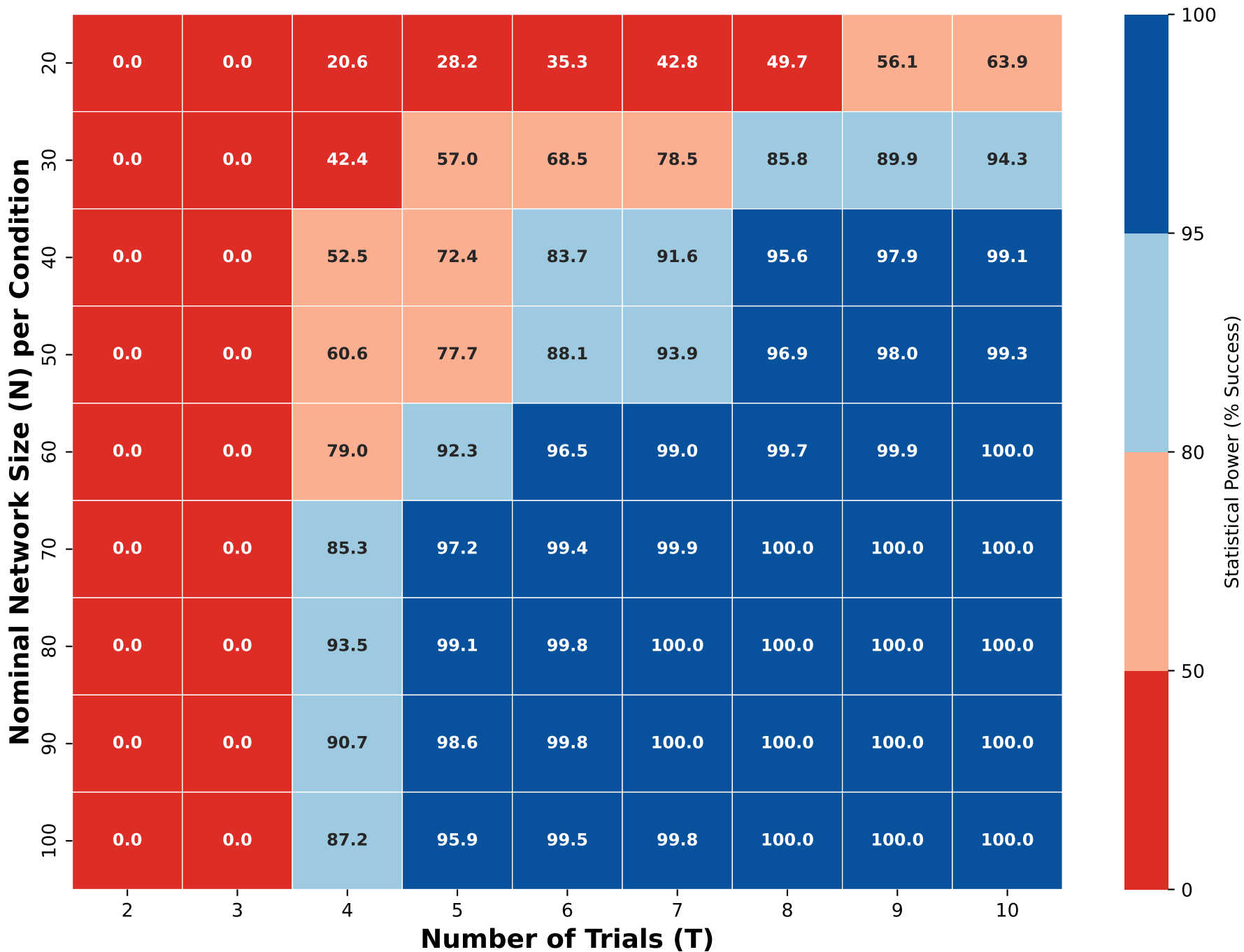
Statistical Power (%) Congenial_Count - Left Users (K=4)
