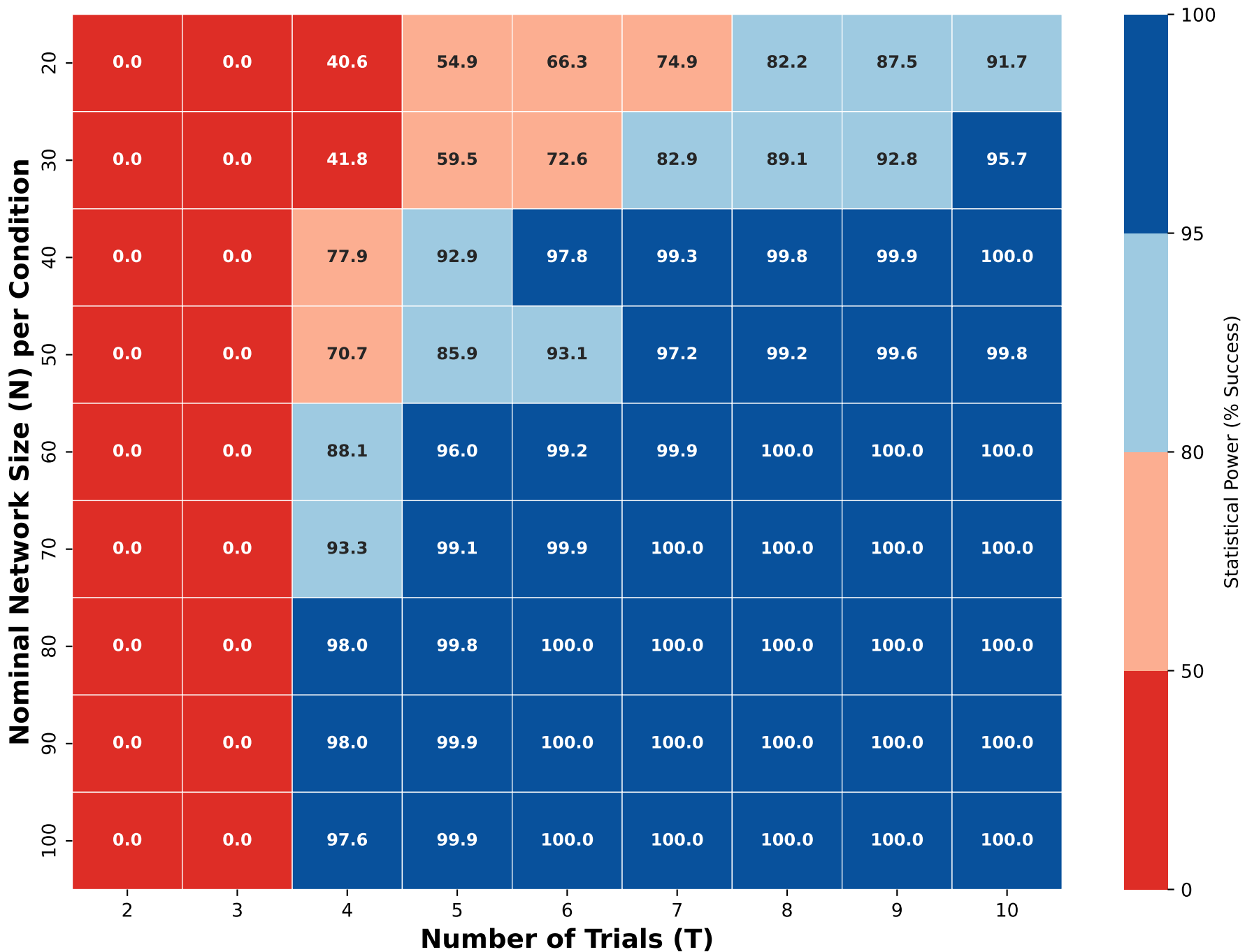
Statistical Power (%) Contrary_Count - Left Users (K=4)
