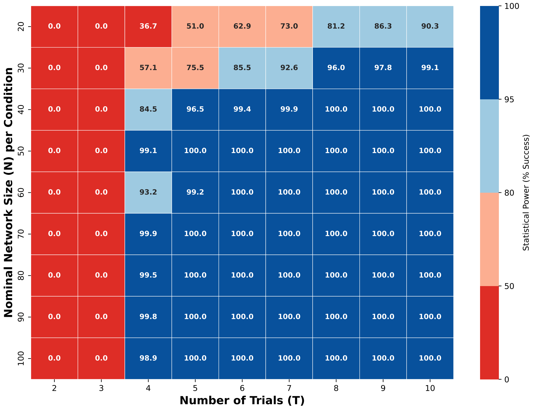
Statistical Power (%) Contrary_Count - Right Users (K=4)
