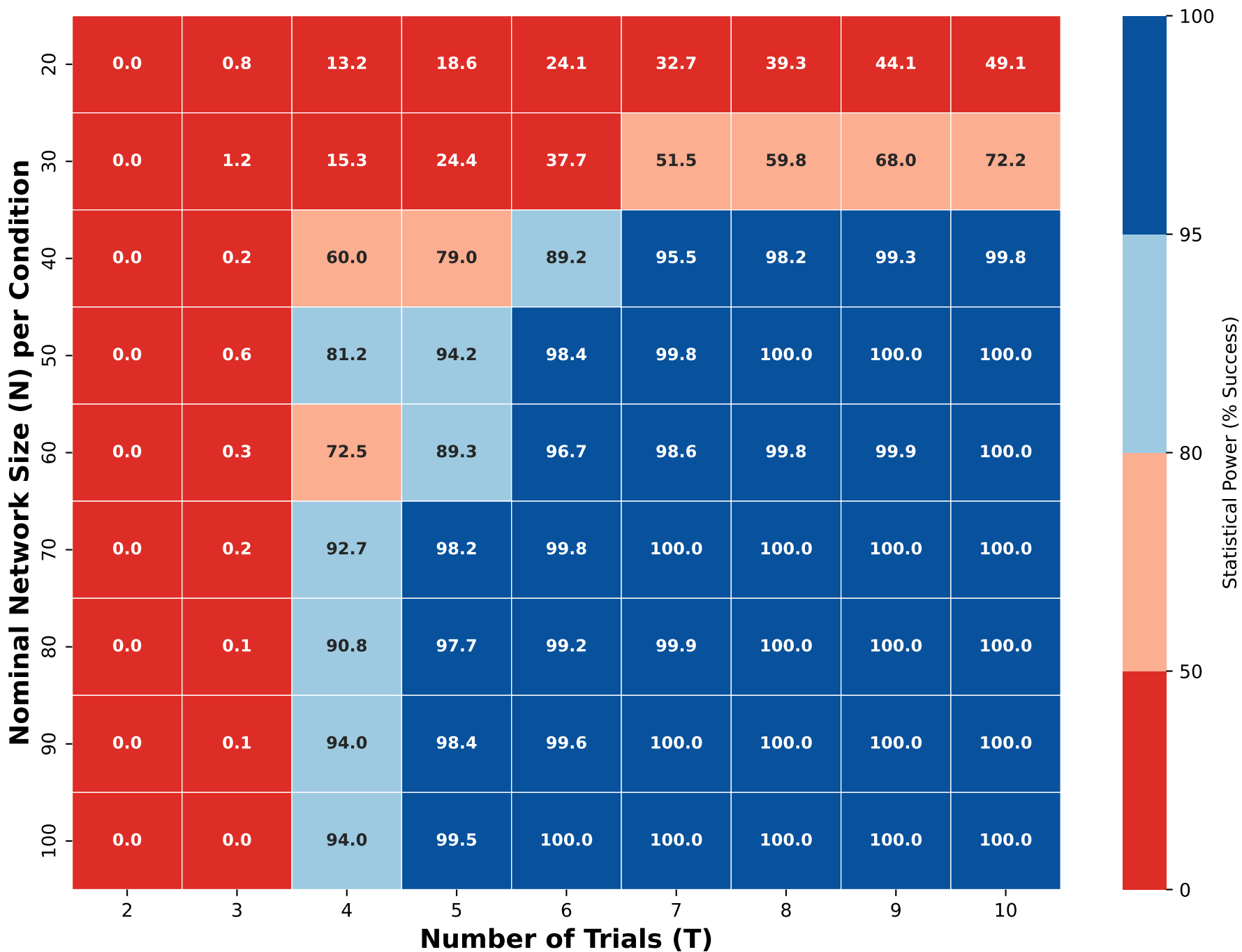
Statistical Power (%) Opposite_EQ_0 - Right Users (K=4)
