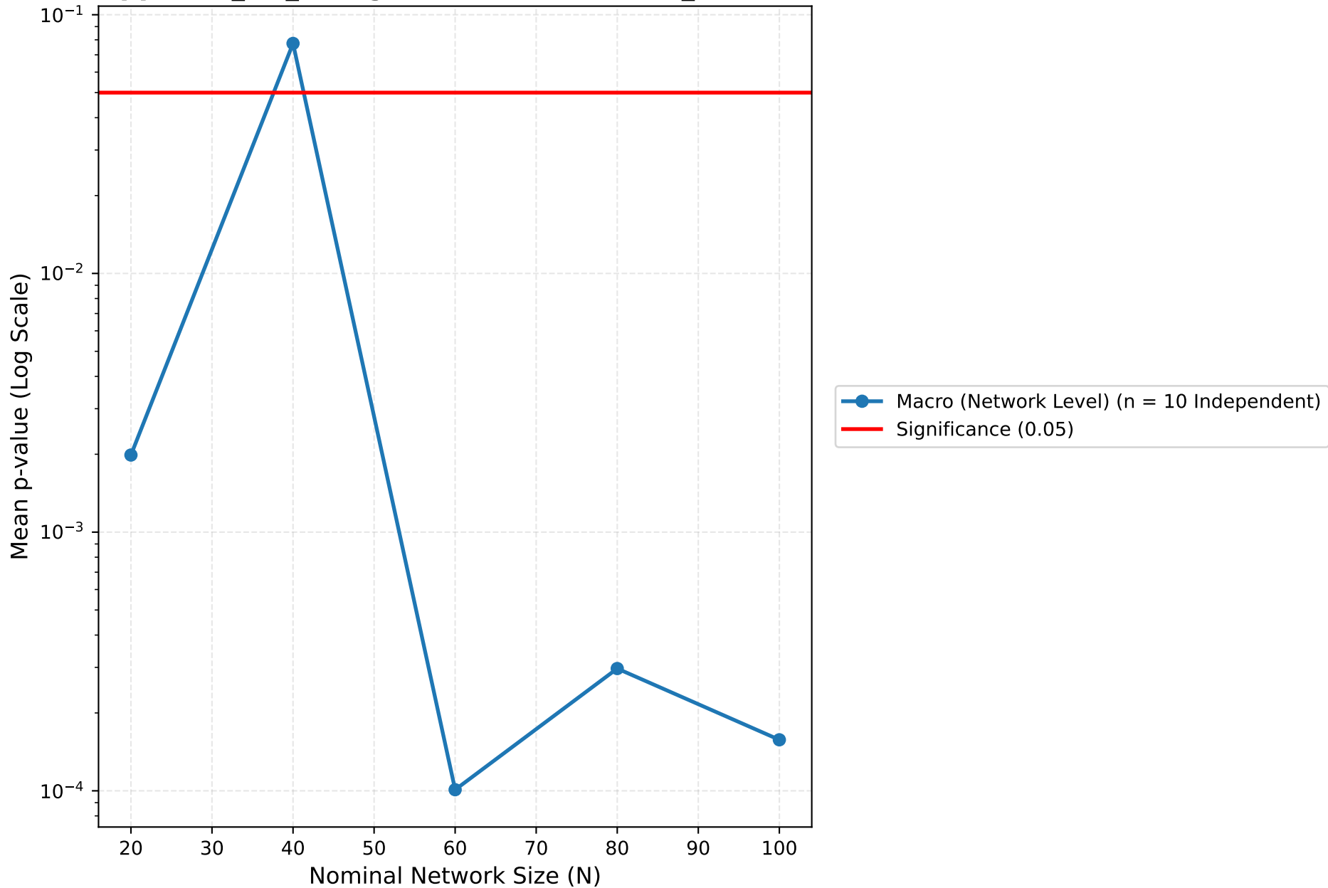
Opposite_EQ_0: Right Users (K=5, Hide_Shared)
