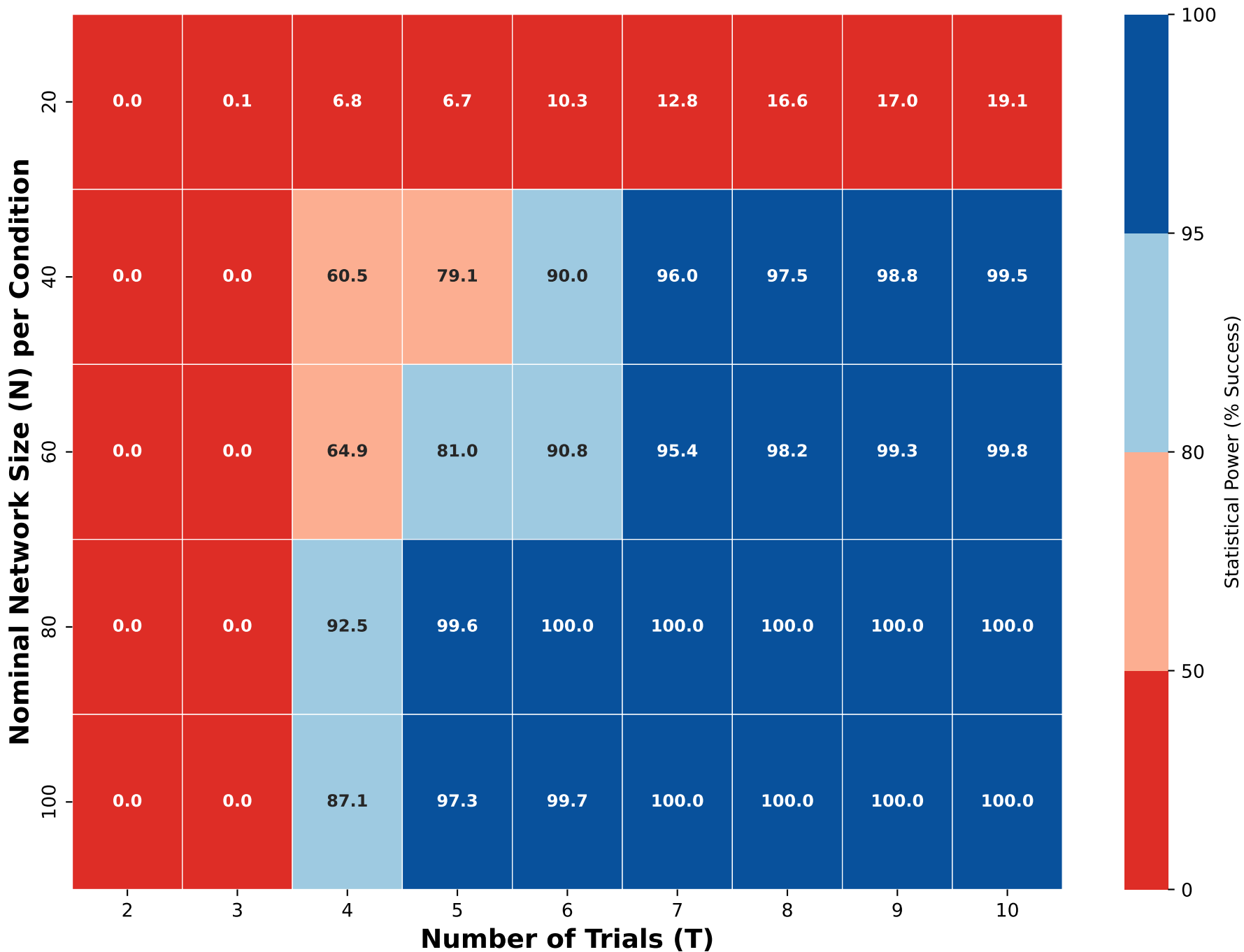
Statistical Power (%) Contrary_Count - Left Users (K=5)
