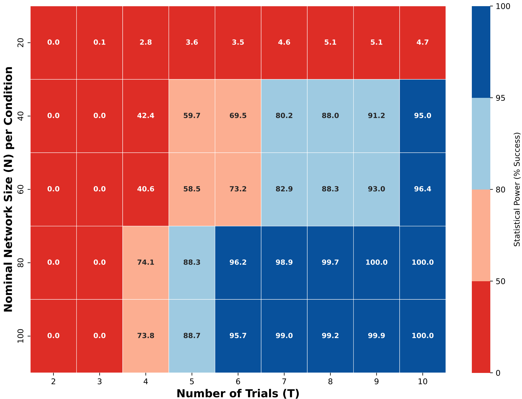
Statistical Power (%) Target_GT_2 - Left Users (K=5)
