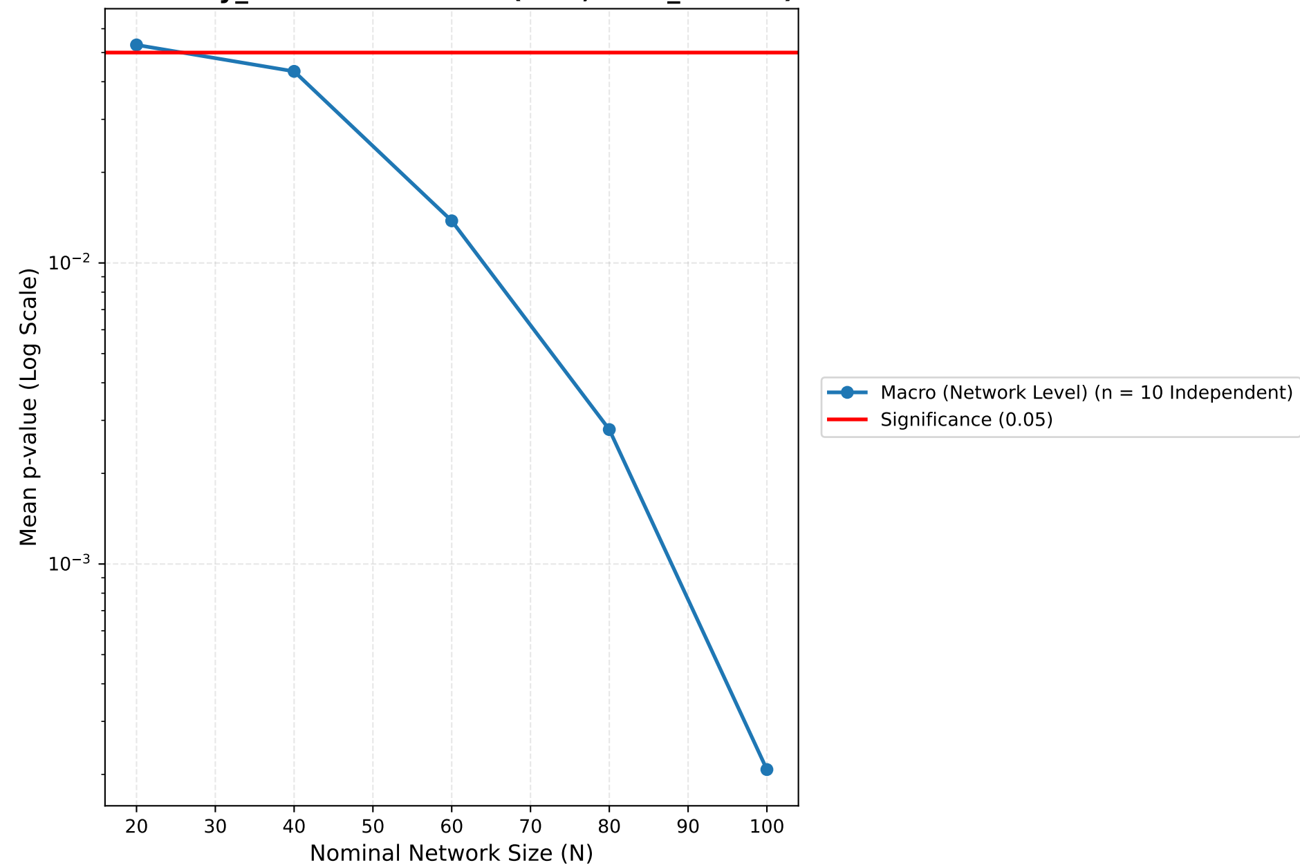
Contrary_Count: Left Users (K=6, Hide_Shared)
