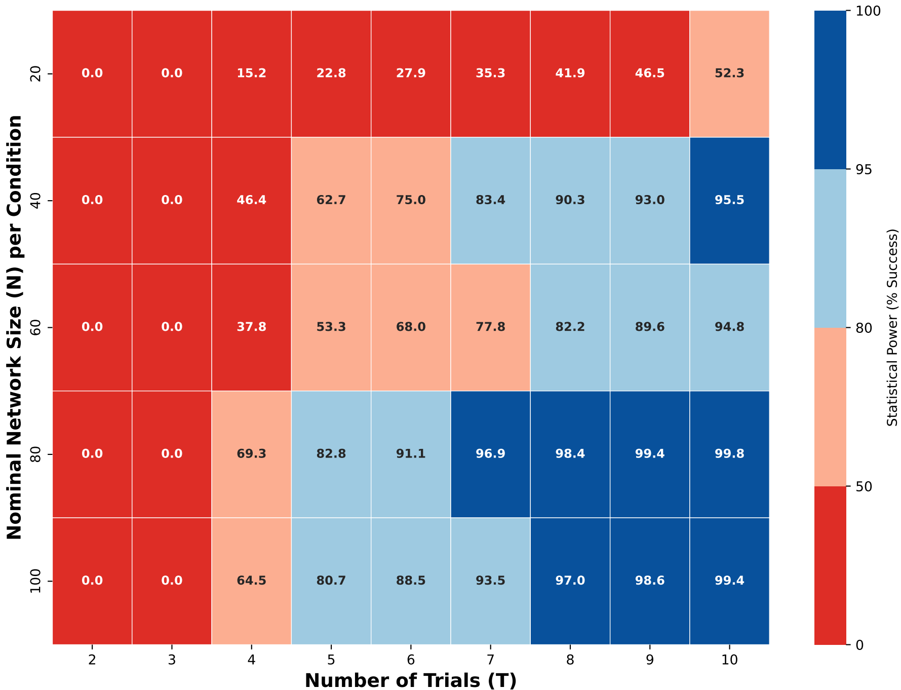
Statistical Power (%) Contrary_Count - Left Users (K=6)
