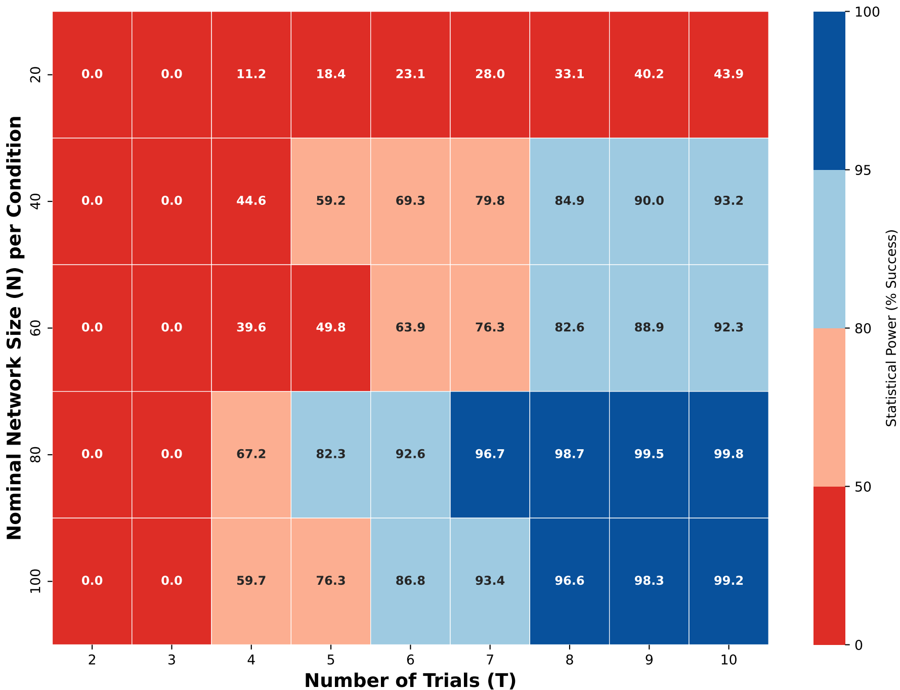
Statistical Power (%) Opposite_EQ_0 - Left Users (K=6)
