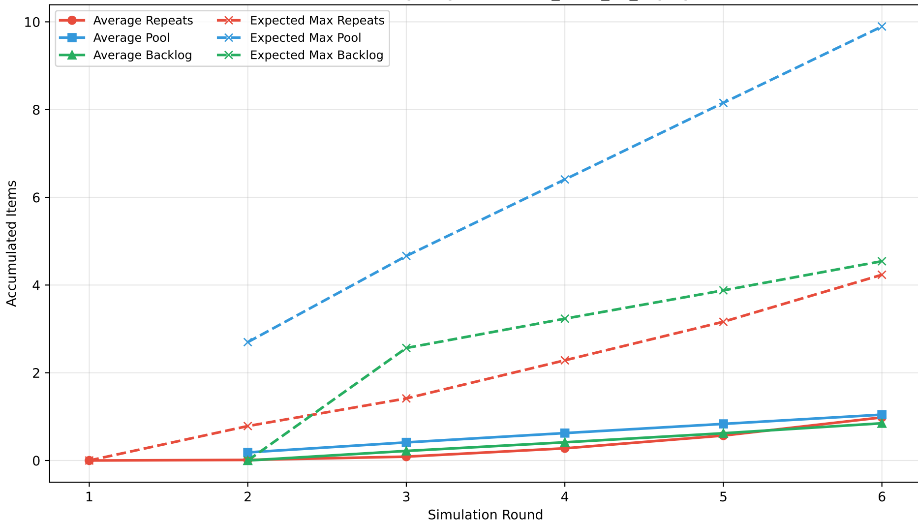
Plot 04: Feed Sourcing Diagnostics (Sim_N100_K4_seggregated)
