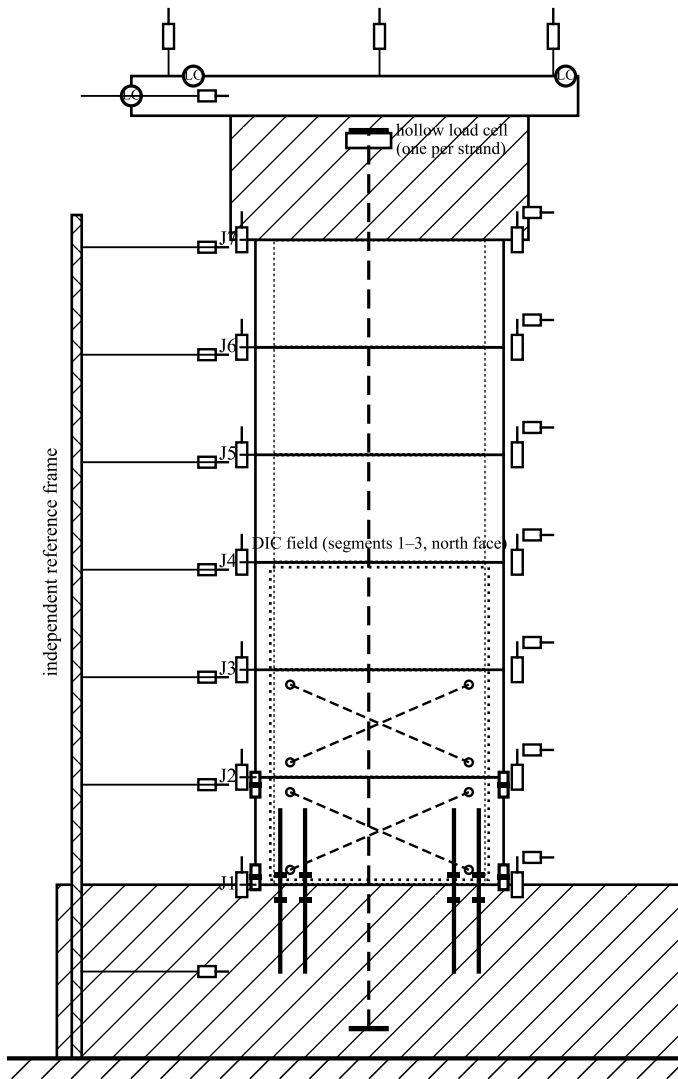
Fig. 4.2 Instrumentation layout on the PS specimen (elevation, bridge longitudinal direction)
