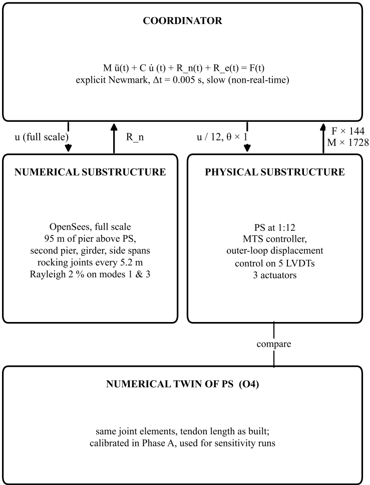
Fig. 4.1 Hybrid-simulation test setup
