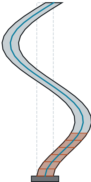
mode 3 T = 0.137 s
