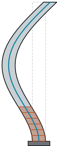
mode 2 T = 0.418 s
