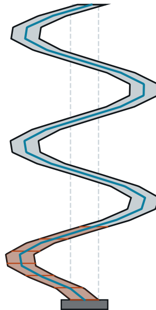
mode 6 T = 0.0259 s
