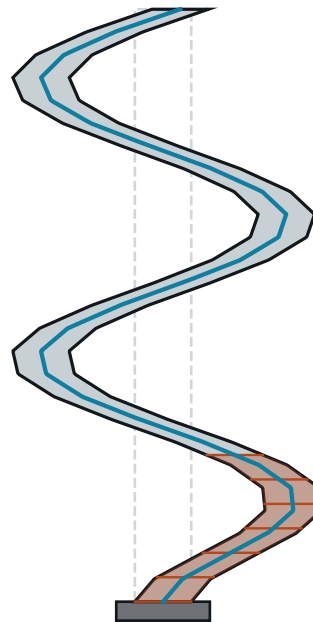
mode 5 T = 0.0393 s
