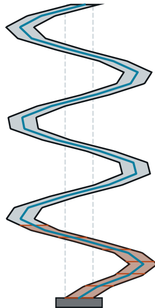
mode 7 T = 0.0183 s
