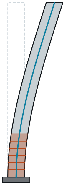
mode 1 T = 3.49 s
