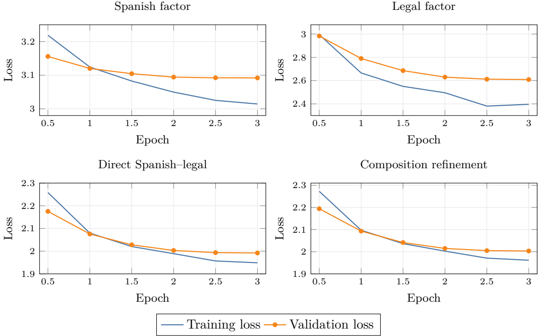
Figure 3: Training and validation loss for the four adapter-training runs. Values are reported at the twice-per-epoch validation schedule. Vertical scales differ across panels.
