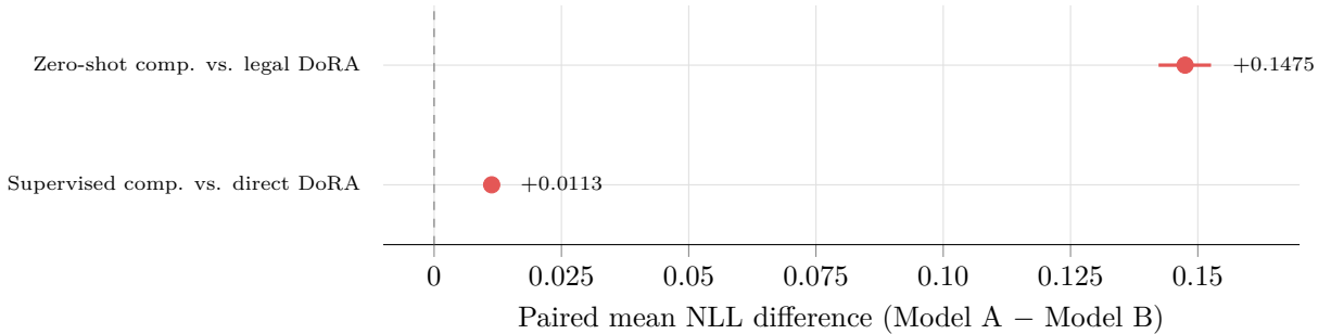
Figure 2: Paired NLL differences for the two composition comparisons. Horizontal lines denote 95% paired-bootstrap confidence intervals; positive values favor the second model named in each row.
