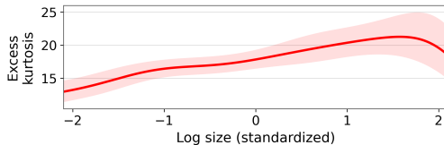
Conditional excess kurtosis
