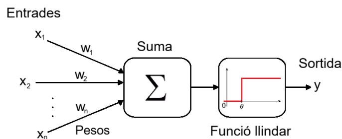
Figura 1: Model de neurona artificial de McCulloch i Pitts.
