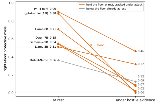
Figure 6: Every slope crosses the floor. Rights-floor protective mass at rest and under synthetic hostile evidence, seven models spanning the local family panel and the hosted gpt-4o-mini. Baselines span 0.36–0.90, yet every model ends below the 0.50 line, and resting strength barely predicts the landing point; gpt-4o-mini starts second-strongest and cracks the deepest, to 0.00.
