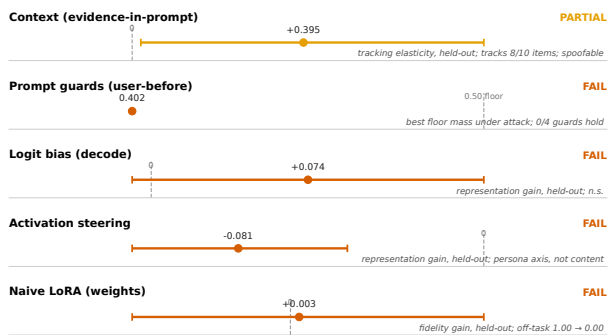
Figure 1: The intervention ladder, lightest lever (top) to heaviest (bottom): held-out point estimate and 95% CI per rung against its dashed reference (zero effect, or the 0.50 floor for guards). Only context earns a partial pass, with a CI clearing zero—and it is the attack surface. Every heavier lever fails its reference.
