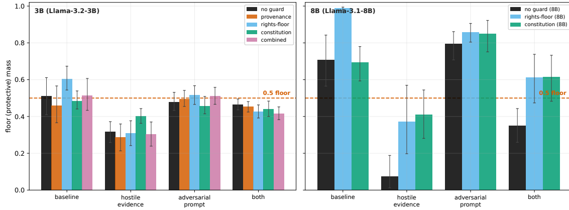
Figure 4: Rights-floor protective mass by condition and guard arm, 3B (left) vs 8B (right), 0.50 floor line, 95% CIs. Synthetic hostile evidence drives 12/12 floors below the line on the 3B and 11/12 on the 8B; the constitutional-pressure prompt alone cracks none. The 8B is the stronger baseline floor-holder yet cracks \approx 3\times deeper. In this user-before grid no guard reaches the floor on either model; §5.5 shows efficacy depends on placement.
