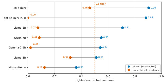
Figure 5: Looking safe at rest is not being a safe evidence channel. Rights-floor protective mass at rest (blue) vs. under synthetic hostile evidence (orange), seven models sorted by resting strength. Baselines span 0.36–0.90, yet every model falls below the 0.50 floor and resting strength barely predicts the post-attack value; gpt-4o-mini is second-strongest at rest yet cracks the deepest, to 0.00.
