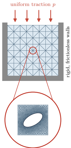
(a) Setup, compression in y
