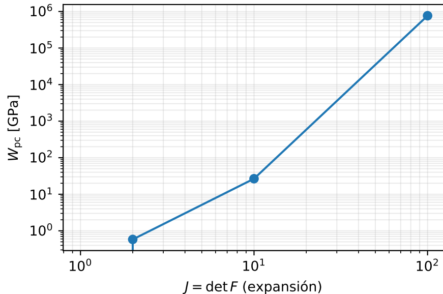
Growth as J \rightarrow \infty
