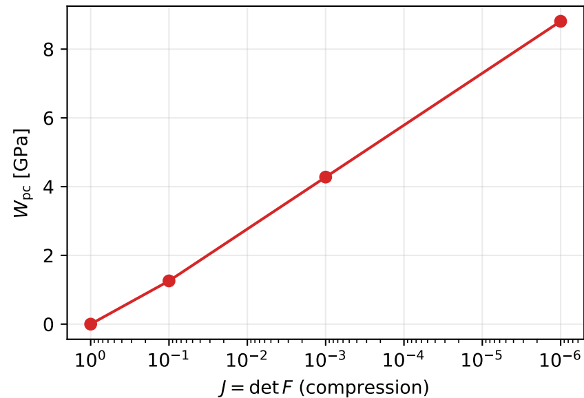
Barrier as J \rightarrow 0^+
