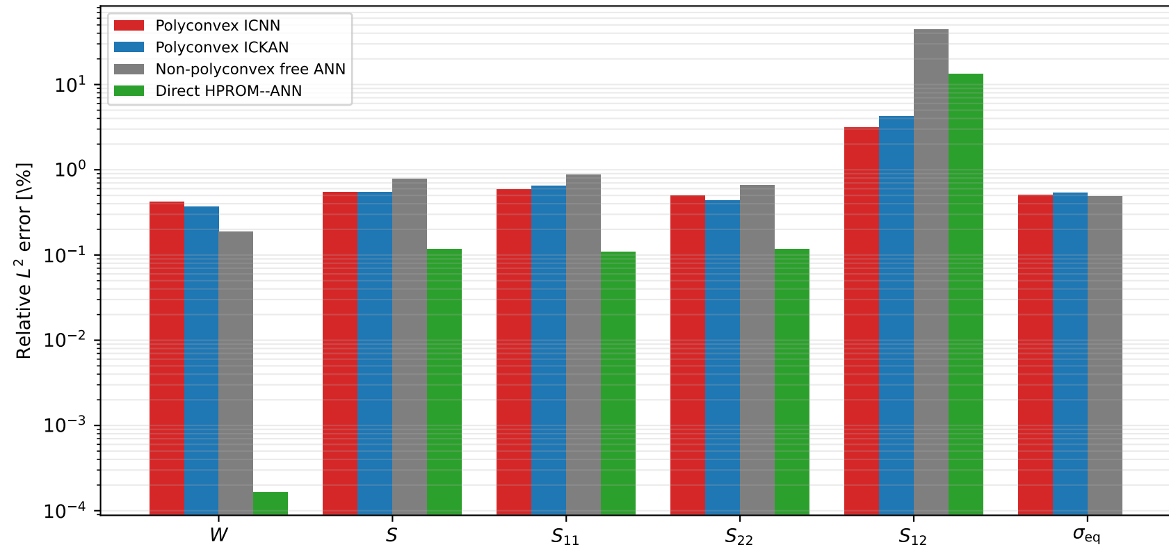
Stage--10 accuracy: certified models vs. non-polyconvex baseline vs. direct HPRM--ANN
