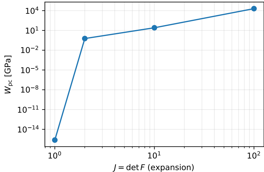
Growth as J \rightarrow \infty
