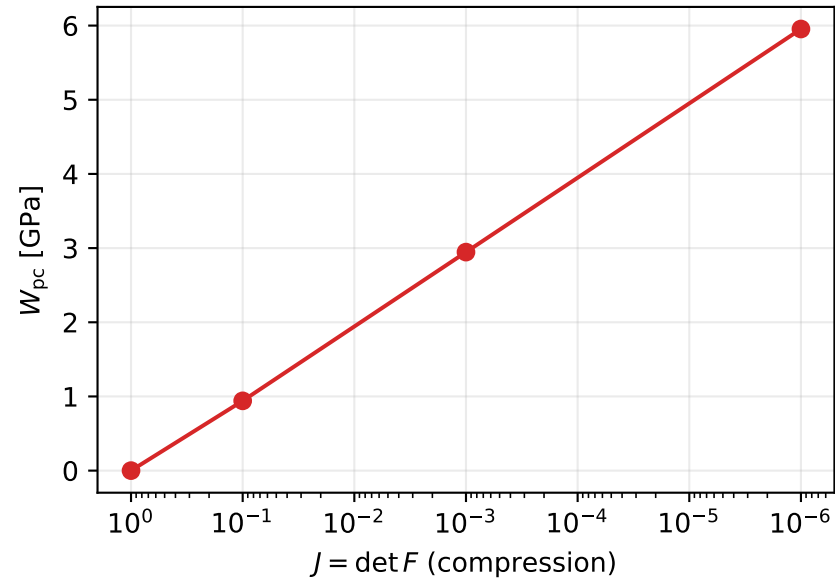
Barrier as J \rightarrow 0^+
