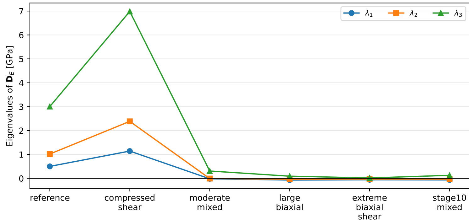
FOM energy-Hessian audit: \mathbf{D}_E = \partial^2 W / \partial \mathbf{e}^2
