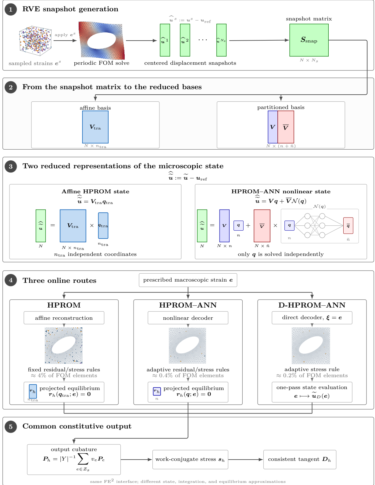
Figure 4: Intrusive reduced references used in the structural comparison. FOM snapshots provide either an affine state representation or a primary–secondary partition in which the ANN predicts the secondary coordinates. Online, HPROM and HPROM–ANN solve projected equilibrium with fixed and adaptive cubature, respectively, whereas D-HPROM–ANN evaluates the nonlinear decoder directly. All three retain microscopic constitutive evaluations and return the same stress–tangent interface.
