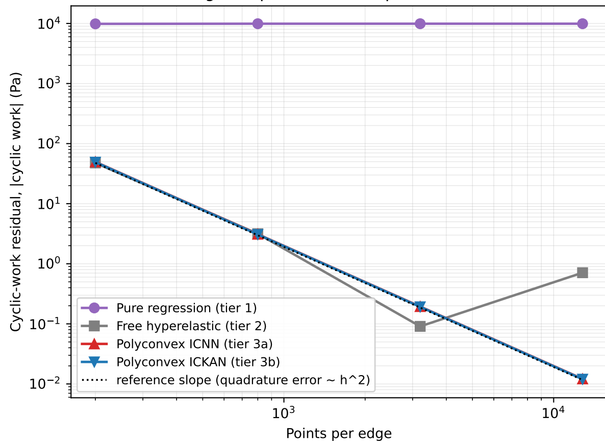
Mixed-triangle loop: residual vs. quadrature refinement
