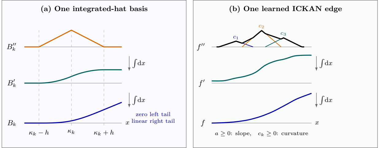
Figure 4: Integrated-hat parameterization of an ICKAN edge. (a) A localized nonnegative curvature hat integrates to a nonnegative slope and a convex C^2 basis with a zero left tail and a linear right tail. (b) Nonnegative learned coefficients combine several fixed bases into a nonnegative edge curvature; integration gives a nondecreasing slope and a convex, nondecreasing connection. The curves illustrate the analytic construction; they do not represent the deployed grid or parameter count.
