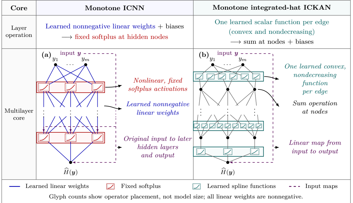
Figure 3: Multilayer monotone cores mapping the conditioned paired features \mathbf{y} to the scalar contribution \hat{H}(\mathbf{y}) . (a) The ICNN learns nonnegative linear maps and applies fixed softplus activations at hidden nodes. (b) The ICKAN learns one convex, nondecreasing scalar function per edge and sums them at nodes. Purple dashed paths denote nonnegative maps of the complete input; ellipses denote intervening layers. Glyph counts indicate where each operation acts, not deployed widths or parameter counts. Unrestricted biases are omitted, and the diagram represents the neural cores rather than the complete energy.
