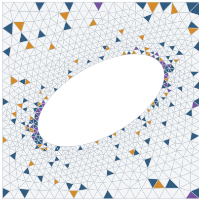
HPROM 135 residual / 73 stress 183 distinct elements
