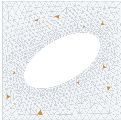
D-HPROM-ANN 0 residual / 10 stress 10 distinct elements
