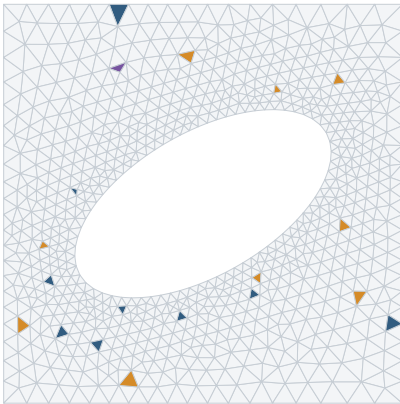
HPROM-ANN 10 residual / 10 stress 19 distinct elements
