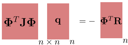
(b) Galerkin-PROM Newton system
