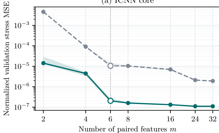
(a) ICNN core
