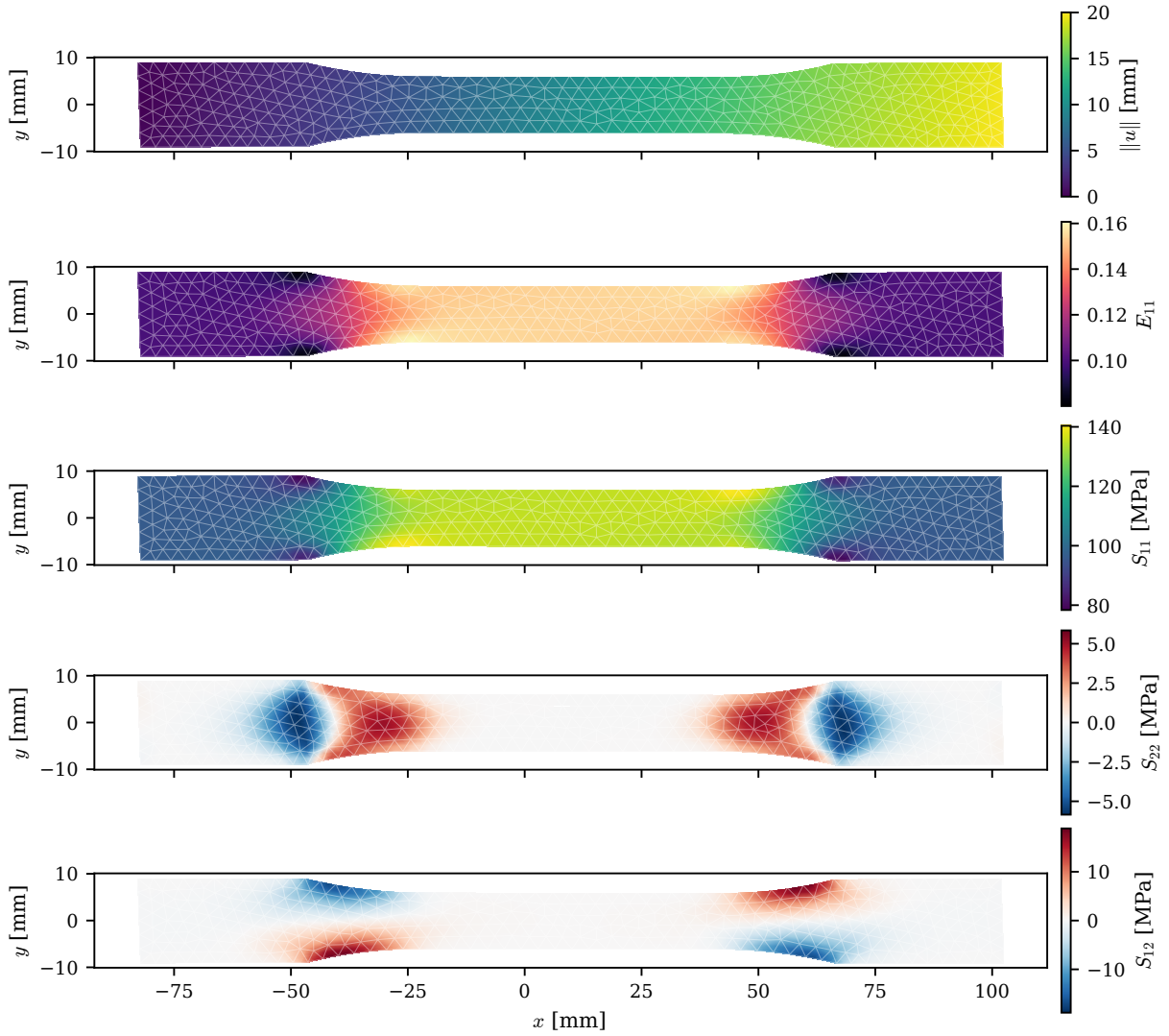
Figure 8: Nested FOM-FE 2 reference at 100 kN per end. Fields are displayed on the actual deformed mesh, without displacement amplification. Gauss-point strain and stress values are first averaged within each element and then patch-averaged to nodes for visualization only. These recovered contours are not the raw fields used in error norms and can smooth local extrema. Stresses are second Piola components. A three-dimensional von Mises stress is not reconstructed because the saved output does not include the necessary out-of-plane Cauchy stress.
