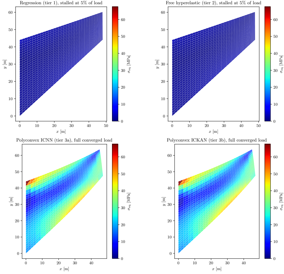
Figure 19: Cook's membrane, equivalent (von Mises) stress field at the same four states as Figure 18, element-constant shading (one value per element, the mean of its three Gauss points). Both certified cores show the expected concentration near the clamped edge; the two uncertified tiers, stalled at 5% of the load, show the correspondingly small field for that load level.
