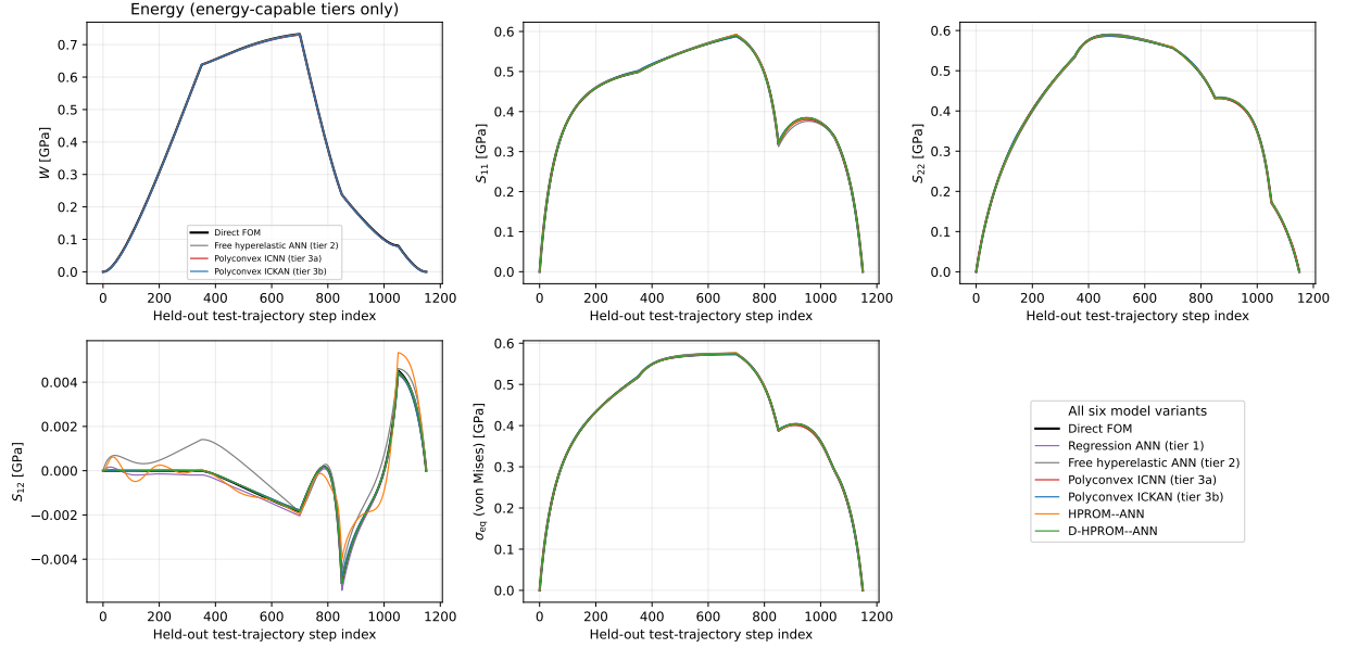
Figure 15: Held-out test-trajectory comparison, direct FOM vs. all six model variants of Table 6 (the tier-1 pure-regression ANN, the tier-2 free hyperelastic ANN, the two certified polyconvex cores, and both HPRM-ANN operating modes): the three second Piola–Kirchhoff components S_{11} , S_{22} , S_{12} and the von Mises equivalent \sigma_{eq} , each shown for all six variants, plus energy W , shown only for the three energy-capable tiers (tier 2, tier 3a, tier 3b): the tier-1 pure-regression model and both HPRM-ANN modes recover stress directly, without an underlying scalar potential, so no energy curve exists for them to plot (Section 4.2.1 for tier 1; Section 6.3’s discussion of the reaction-force procedure for the two HPRM-ANN modes). Every plotted variant is visually indistinguishable from the FOM and from each other on this held-out path (including the free model, whose lack of a polyconvexity certificate is not visible here), which is exactly why Sections 4.2.1 and 6.5 audit them directly (cyclic work, rank-one curvature) rather than relying on this figure.
