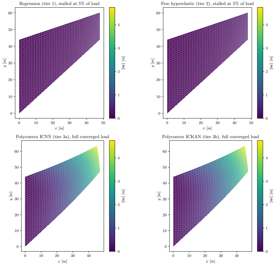
Figure 18: Cook's membrane, deformed states reached by all four PANN tiers, colored by displacement magnitude (reference configuration: Figure 17). Both certified cores (tiers 3a, 3b) reach the full 2.08 \times 10^8 N load with a visibly large bend; the two uncertified tiers, stalled at just 5% of that load, are barely displaced at all.
