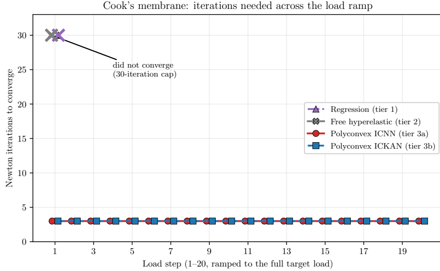
Figure 21: Newton iterations needed at every one of the 20 ramped load steps (tiers 3a and 3b, coincident throughout, offset slightly for legibility). The certified cores need exactly three iterations regardless of load; the two uncertified tiers fail to converge already at the first, smallest step.
