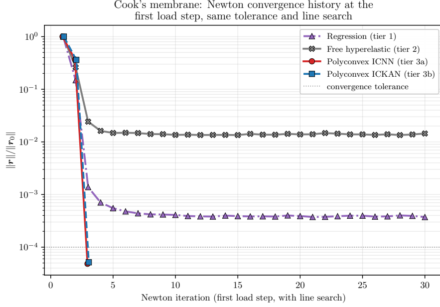
Figure 20: Newton residual history at the first load step, same tolerance and line search for all four tiers (tiers 3a and 3b offset slightly and drawn with distinct markers, since they are otherwise nearly indistinguishable). The certified cores converge in three iterations; the tier-2 free model's residual stalls flat at 1.4% of its initial value, and the tier-1 regression model's stalls, less flatly, at 3.7 \times 10^{-4} .
