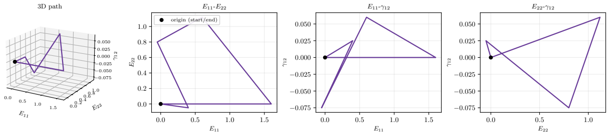
Figure 4: The held-out test trajectory in strain space: one 3D view and three pairwise 2D projections of the same 1 151-state path, read directly from the applied-strain sequence used for every reported accuracy number. The path is a small number of straight segments connecting extreme, mixed states and returning to the origin, visually distinct from the area-sweeping training trajectories of Figure 3.
