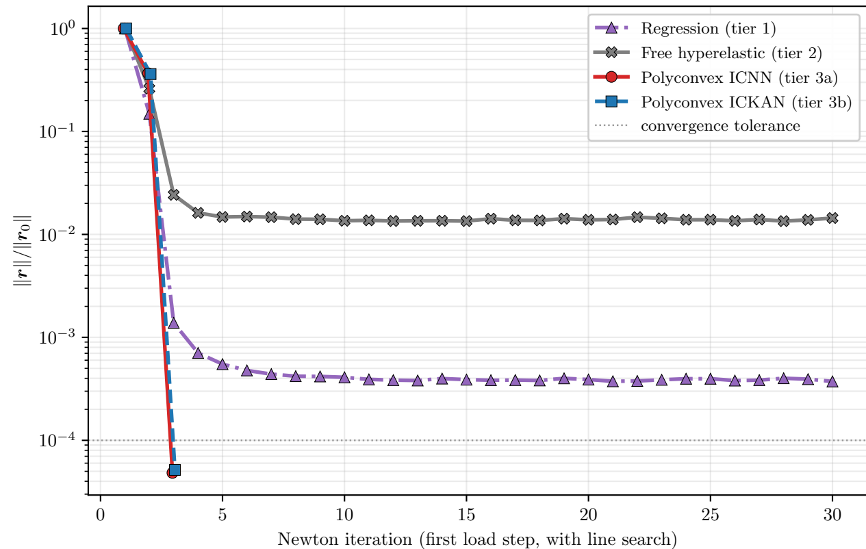
Cook's membrane: Newton convergence history at the first load step, same tolerance and line search
