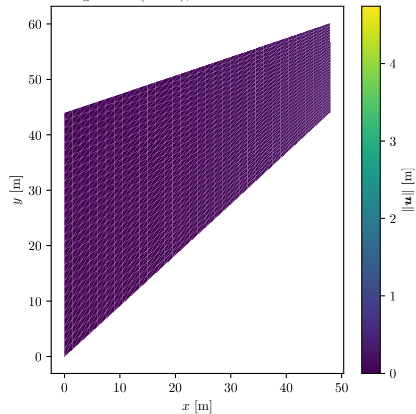
Polyconvex ICNN (tier 3a), full converged load
