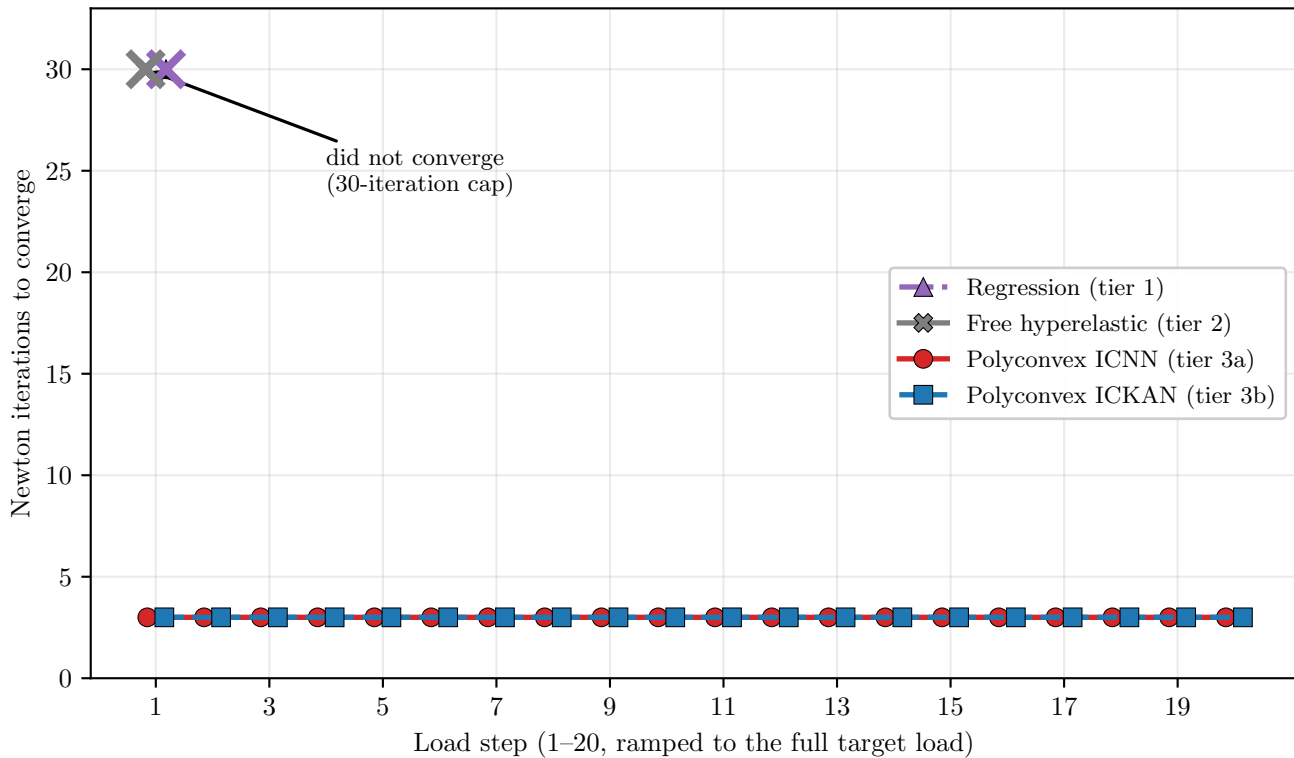
Cook's membrane: iterations needed across the load ramp
