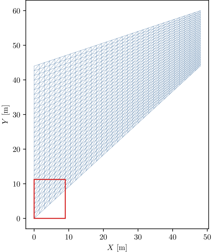
Cook's membrane: reference (undeformed) mesh 512 six-node quadratic triangles (Tri6), 1 536 Gauss points
