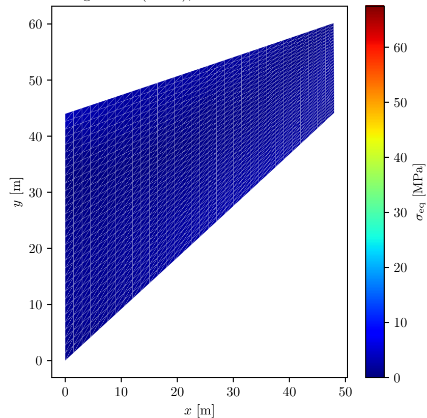
Polyconvex ICNN (tier 3a), full converged load
