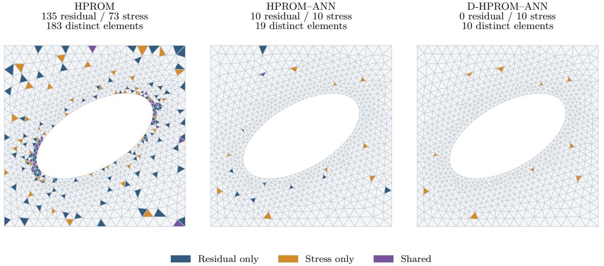
Figure 12: Element supports of the three HPRMs. The pale full-cell mesh provides location context only. Colors distinguish residual-only, stress-only, and shared elements.
