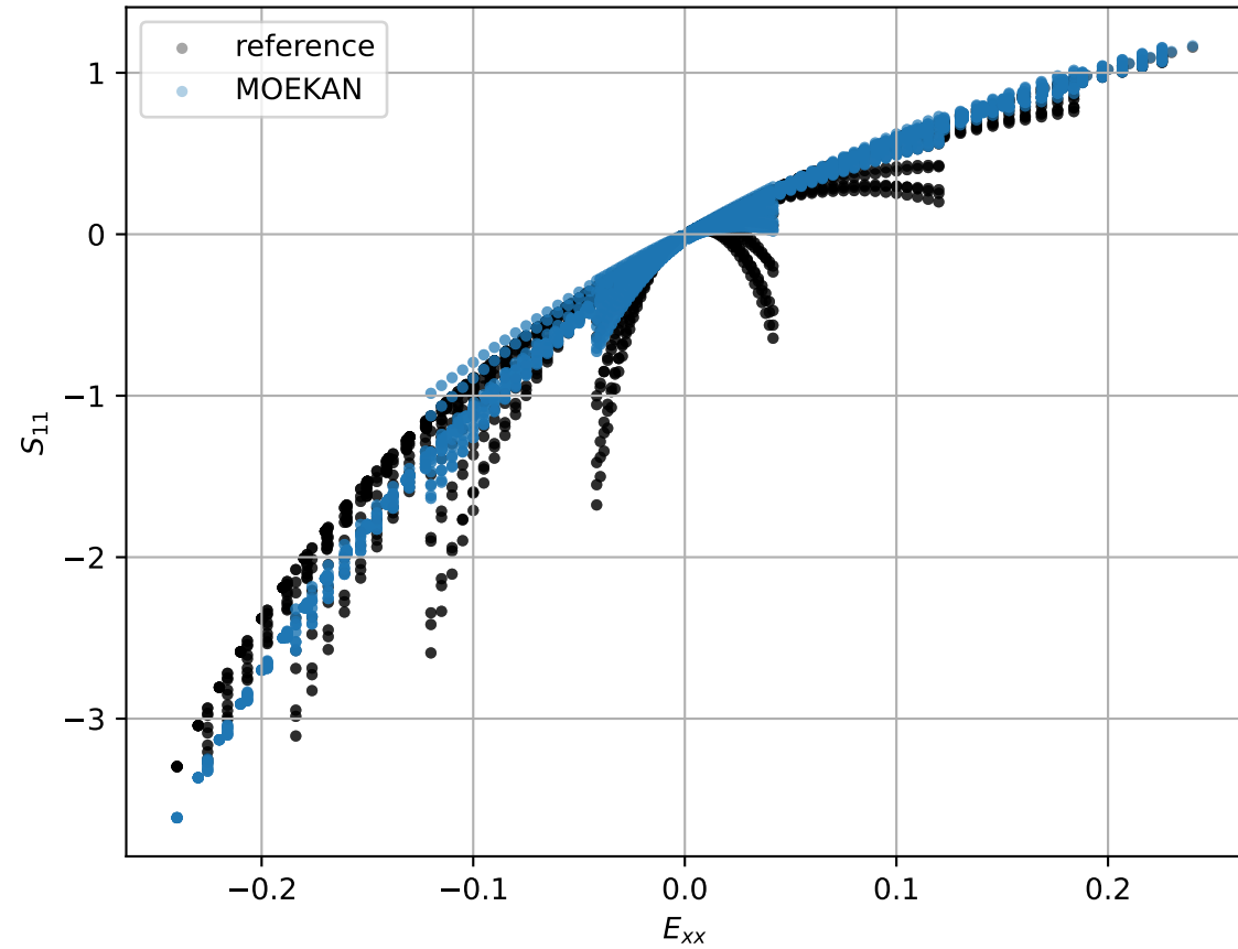
S_{11} versus E_{xx}
