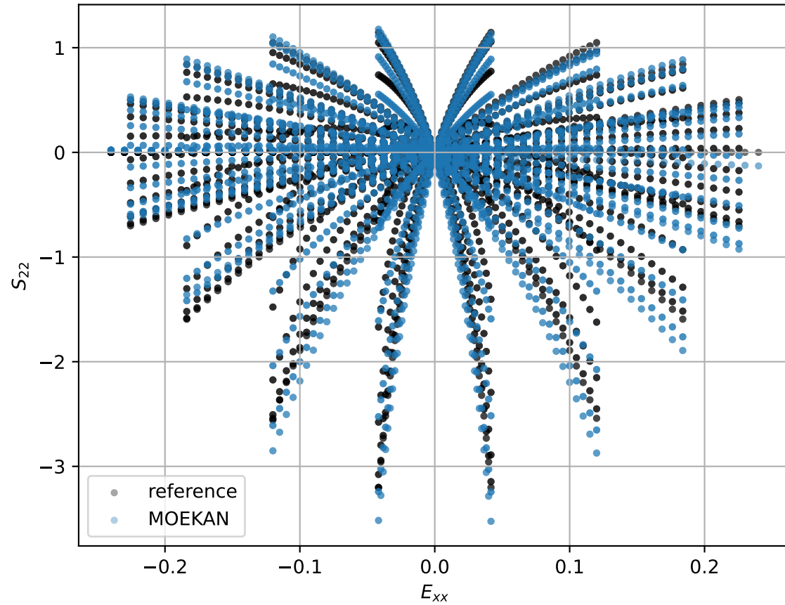
S_{22} versus E_{xx}
