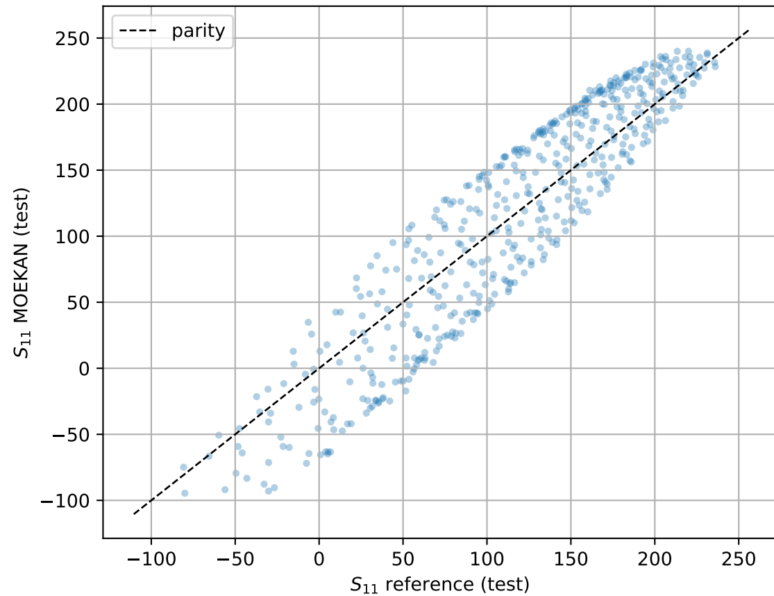
S_{11} parity (test)
