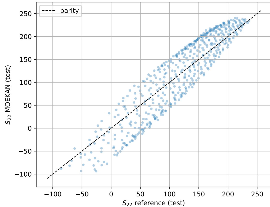
S_{22} parity (test)
