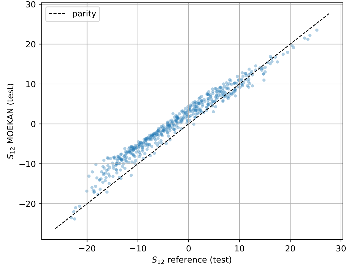
S_{12} parity (test)
