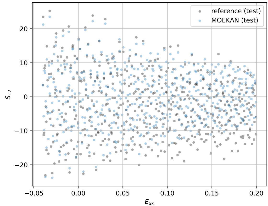
S_{12} versus E_{xx} (test)
