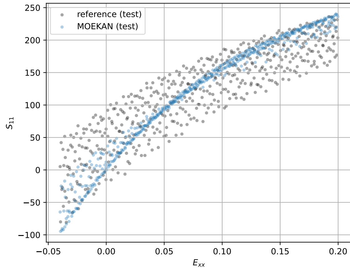
S_{11} versus E_{xx} (test)
