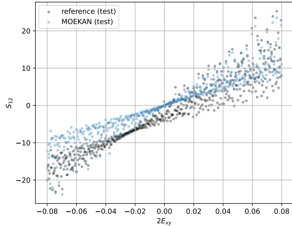
S_{12} versus 2E_{xy} (test)
