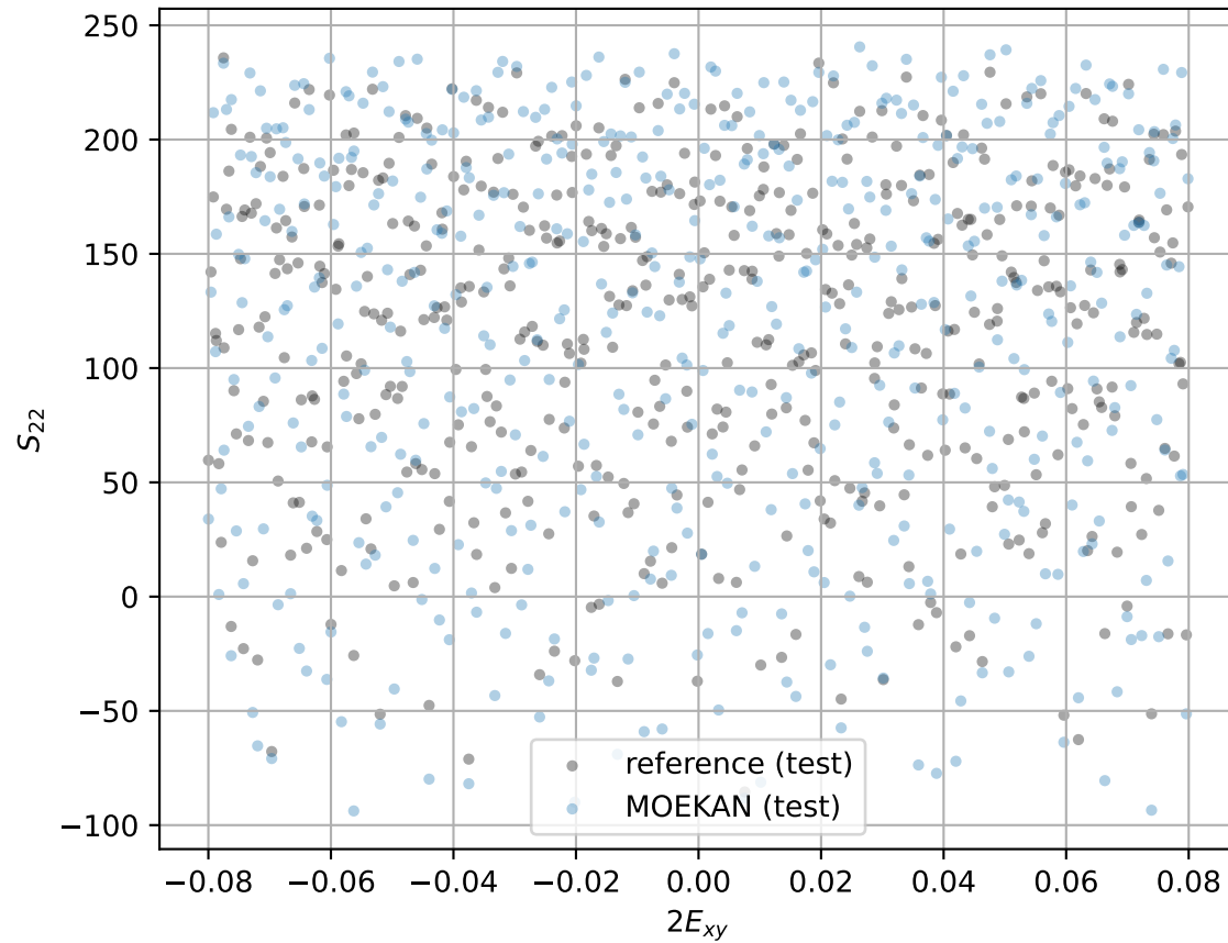
S_{22} versus 2E_{xy} (test)
