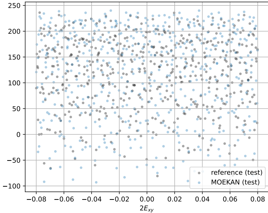
S_{11} versus 2E_{xy} (test)
